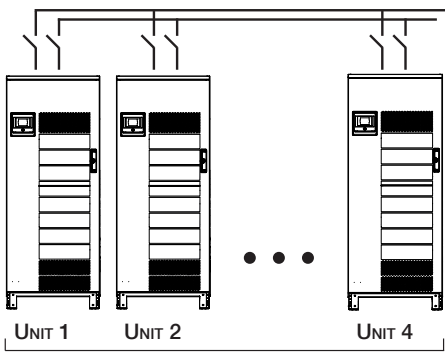
SYSTEM WITH DISTRIBUTED UPSTREAM ARCHITECTURE
